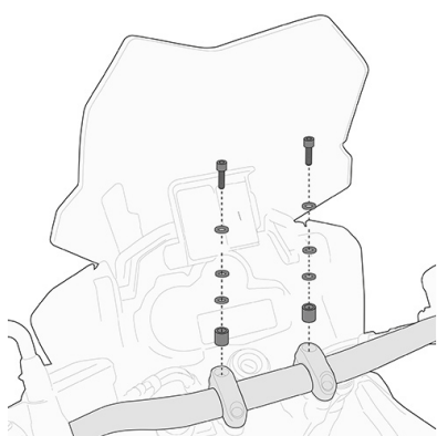
04SKITK Specific kit to mounting the KS900A Smart Bar
